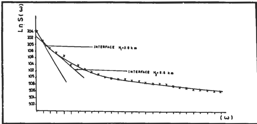
FIG. 4. Local power spectra for interface determination of Um Samiuki area, South Eastern Desert, Egypt.
